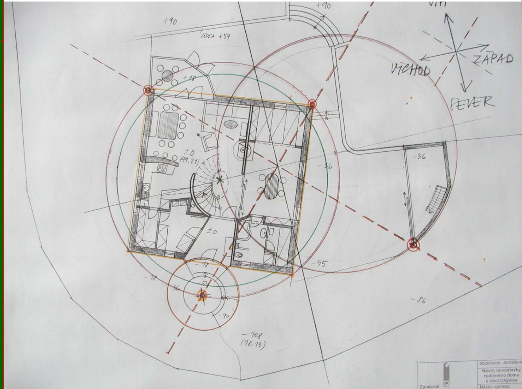
energy efficient house, ground floor plan
